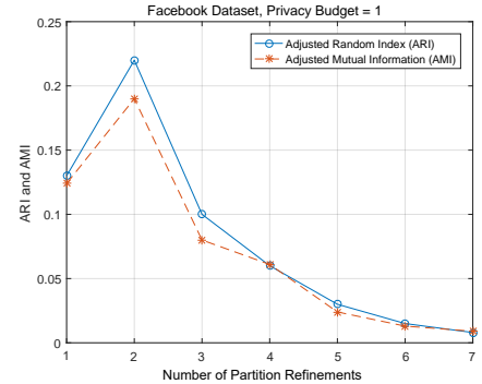
Figure 10: ARI and AMI vs. Number of rounds for grouping refinements (Facebook)
