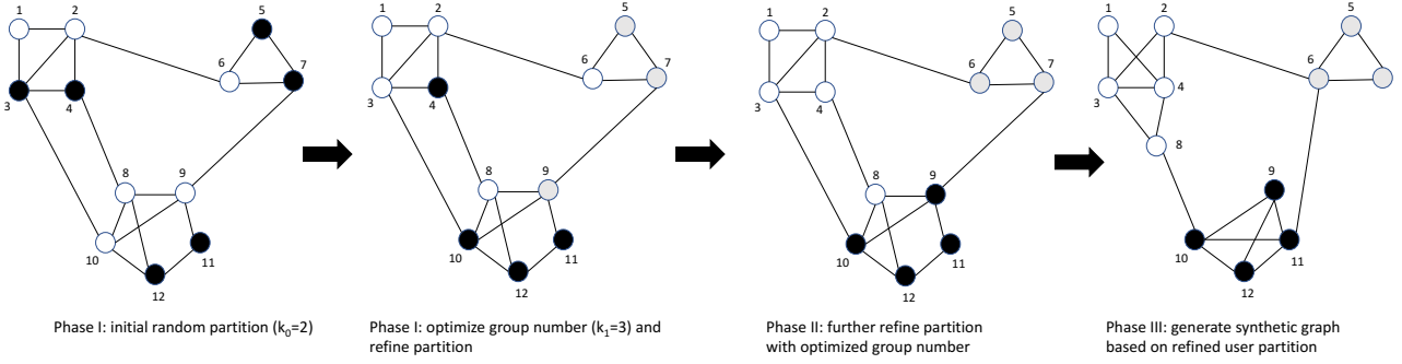
Figure 1: Illustrative example of LDPGen
