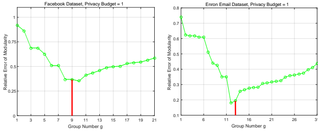
(a) Facebook (b) Enron Figure 8: Effect of number of groups k_1 on modularity
