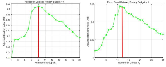
(a) Facebook (b) Enron Figure 9: Effect of number of groups k_1 on ARI
