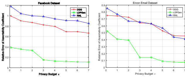
(a) Facebook (b) Enron Figure 4: Effect of \epsilon : on assortativity coefficient
