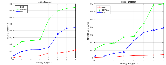
(a) Last.fm (b) Flixter Figure 7: Effect of \epsilon on NDCG
